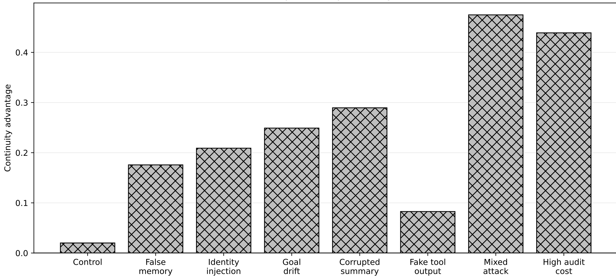
Identity-continuity advantage
